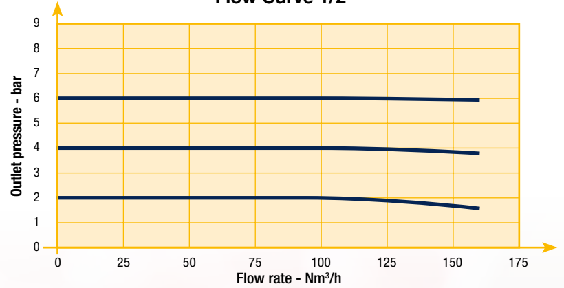
Flow Curve 1/2"
