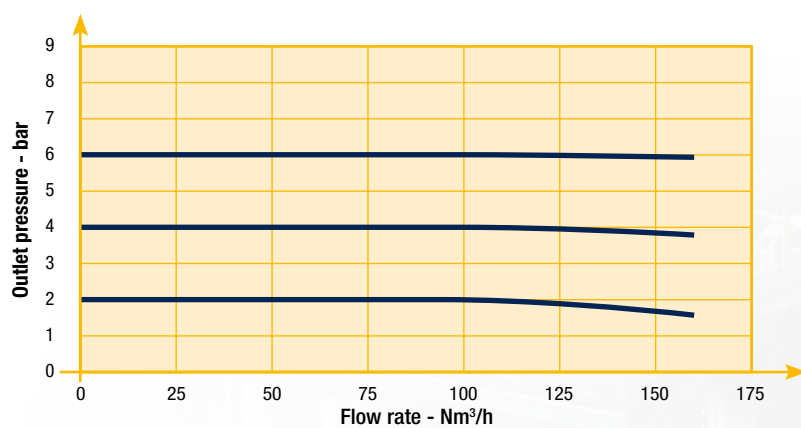
Flow Curve 1/2"
