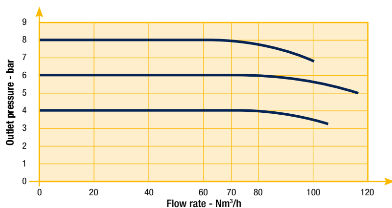
Flow Curve 1/4"
