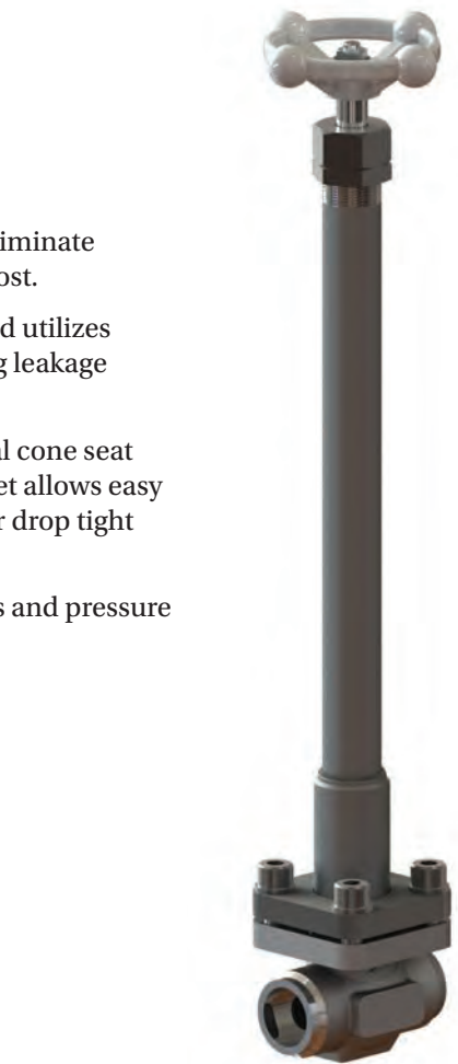
DN15 Stainless Steel Globe Valve Extended Stem with Socket Ends
