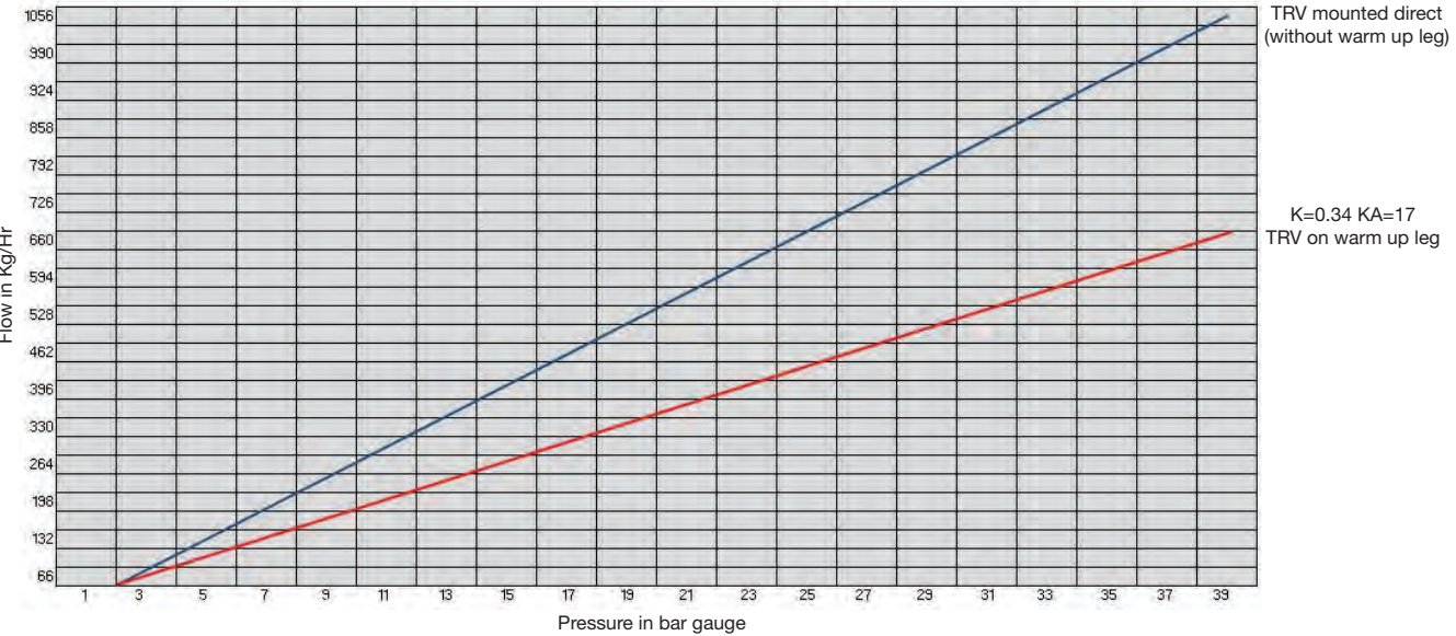
DN6 V2698 Thermal Relief Valve Flow in Kg/Hr @ 0 deg C Inlet & P+10% Area = 50mm squared
