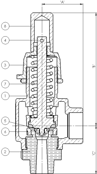
Nozzle 10 Safety Relief Valve
